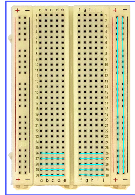
breadboard
